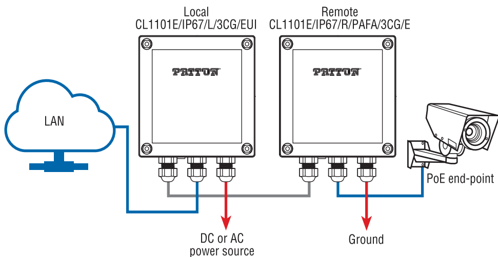
Figure 1. CL1101E/IP67 Ethernet Extender application
